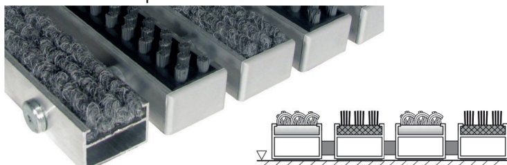
brush strip 3 / grooved PVC x 2
